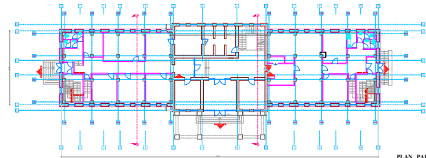
PLAN PARTIER S totala = 676 MP
