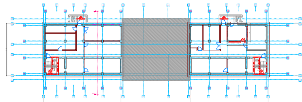
PLAN SUBSOL S totala = 456 MP S terasa Cbh = 228 MP S terasa Vest fara Centrala termica = 208 MP S centrala termica terasa Vest = 20 MP
